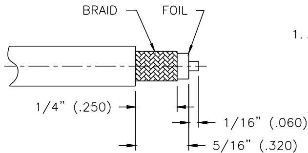
WEATHER SEAL
